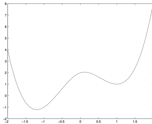
Figure 6.2: Spline interpolation
